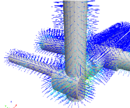
Semmering Base Tunnel – numerical model of the cavern expansion at shaft foot SBT3.1
